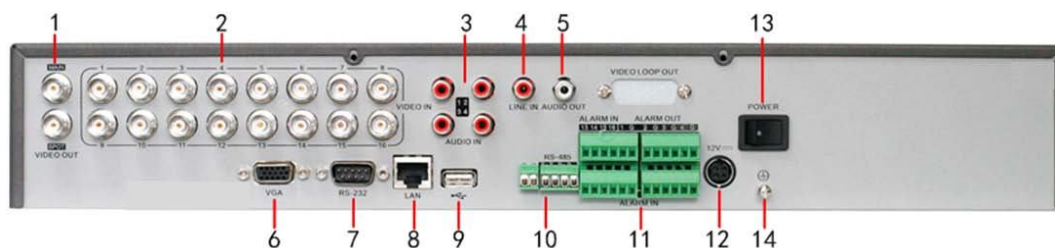
Figure 20. DSR-1605-rw Rear Panel
